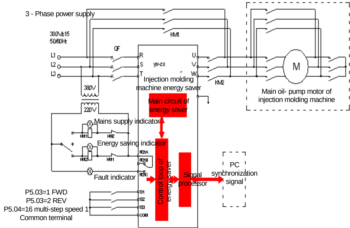
Schematic diagram of connection of injection molding machine with energy saver
